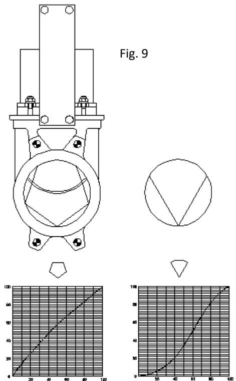
VERTICAL: % MAXIMUM FLOW HORIZONTAL: % OF VALVE OPENING
